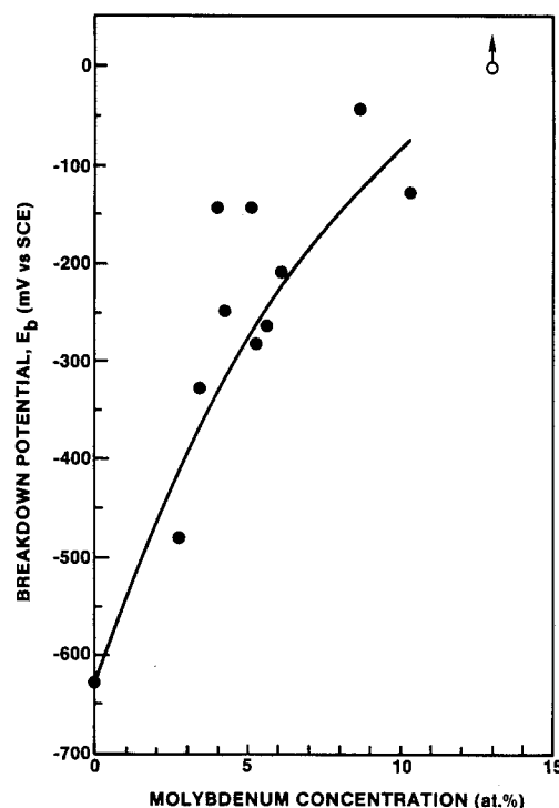
Fig. 6. The effect of the average Mo content in the alloy on the E_b determined from a rapid increase in the current density during potentiodynamic polarization.
